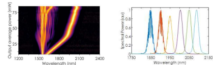
Evolution of the soliton central wavelength vs output average power:
